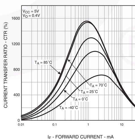
Fig. 9 Current Transfer Ratio vs. Forward Current (6N138 / 6N139 Only)
