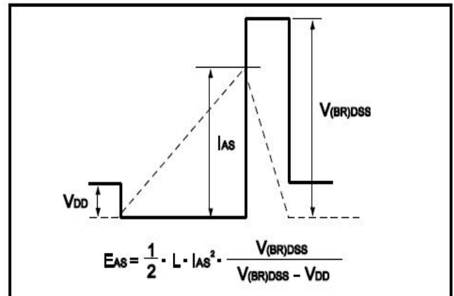
Fig.12 Avalanche Waveform
