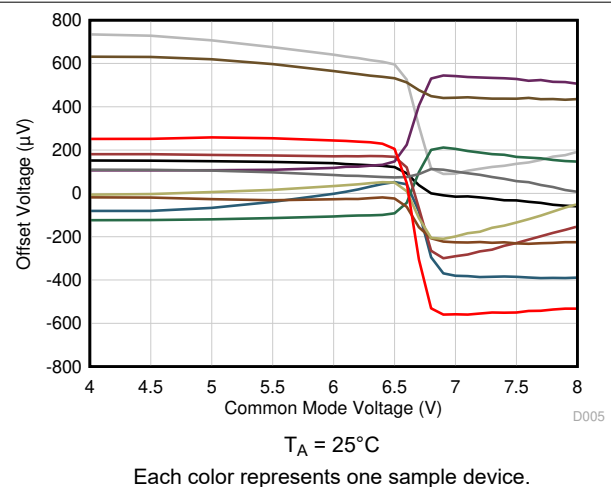
Figure 6-6. Offset Voltage vs Common-Mode Voltage (Transition Region)
