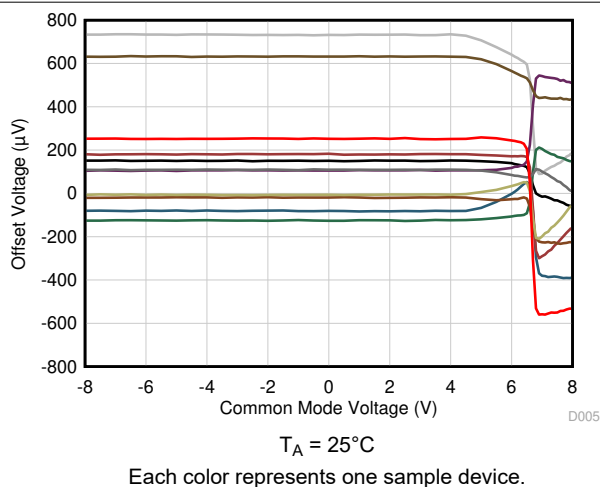
Figure 6-5. Offset Voltage vs Common-Mode Voltage
