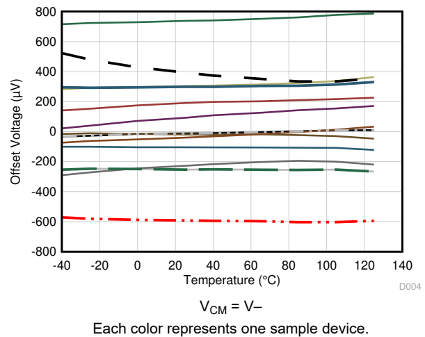
Figure 6-4. Offset Voltage vs Temperature
