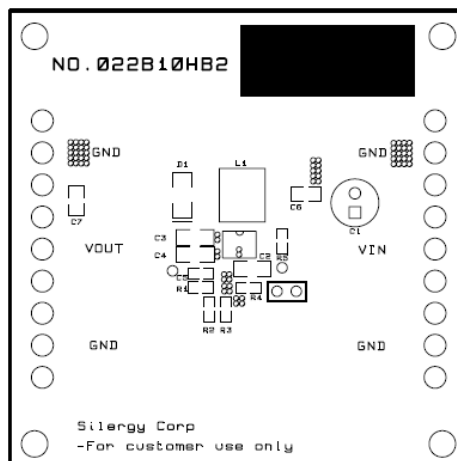
Figure3. Top Silkscreen
