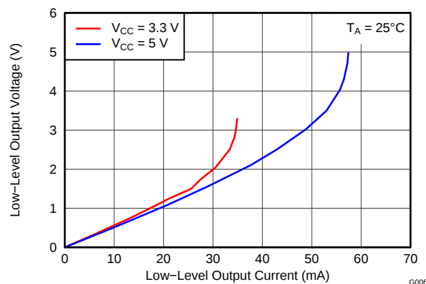
Figure 12. Low-Level Output Voltage vs Low-Level Output Current
