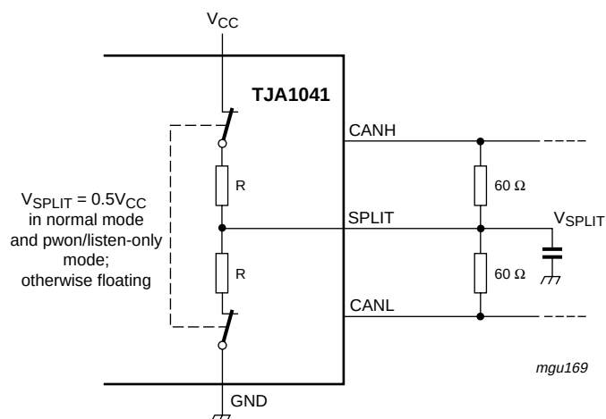
Fig 5. Stabilization circuitry and application
