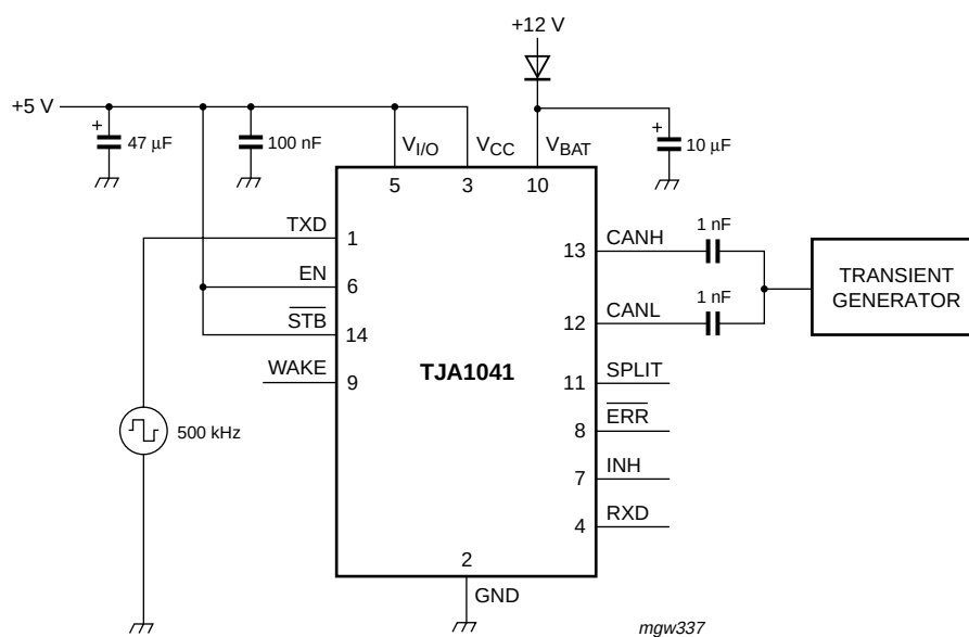
Fig 6. Test circuit for automotive transients
